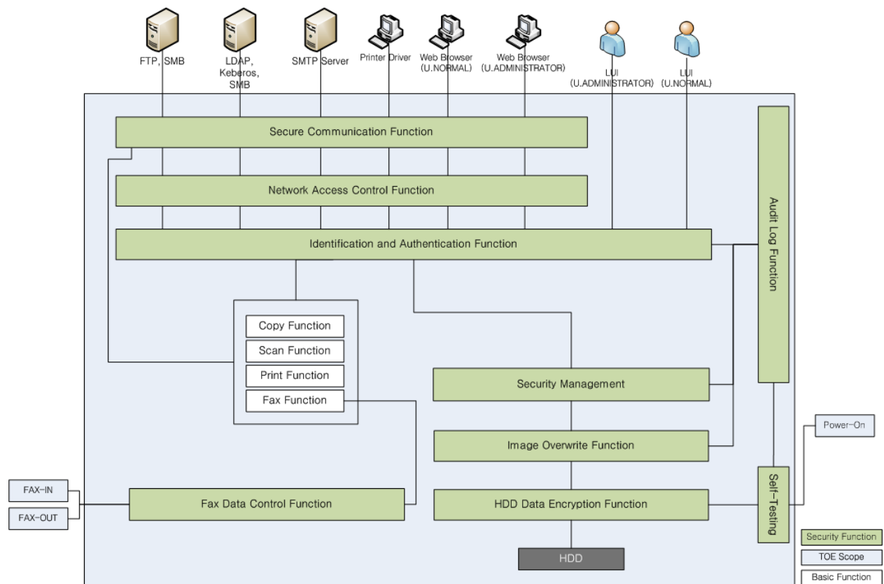
Figure 2: Logical Scope
